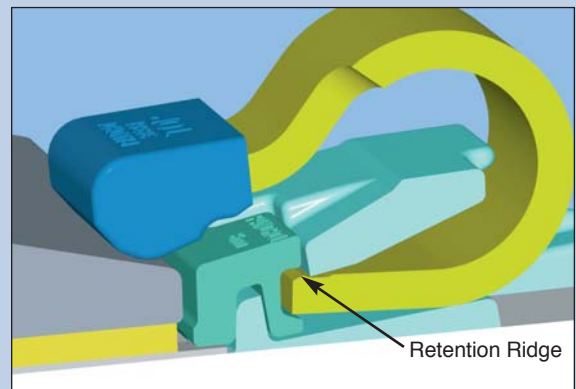
Mechanical lock-in feature provides positive clip retention.
